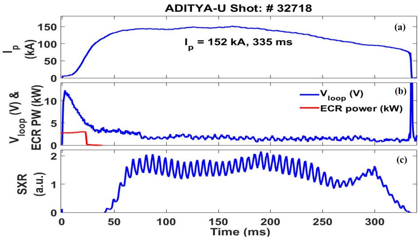
Fig. 1. Temporal evolution of plasma parameters for typical ADITYA-U shot #32718.
